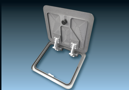
118° opening glue in deck hatch
